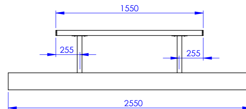
SLAB DIMENSIONS SUGGESTION ONLY
